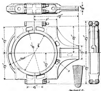
Figs. 1873-1877. Eccentric Strap for Consolidation (2-8-1) Locomotive, American Locomotive Co.
